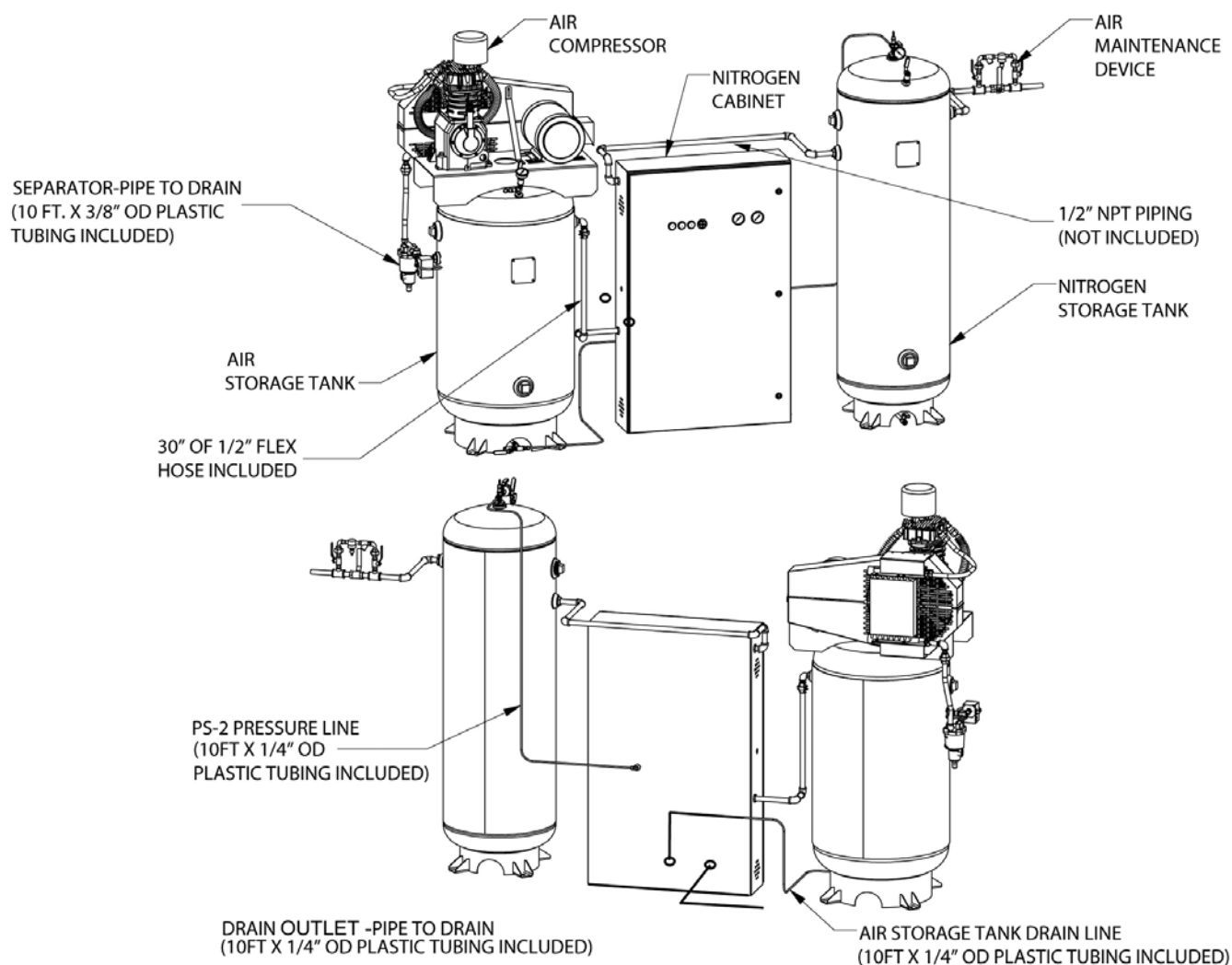
Figure 4: Piping Requirements
