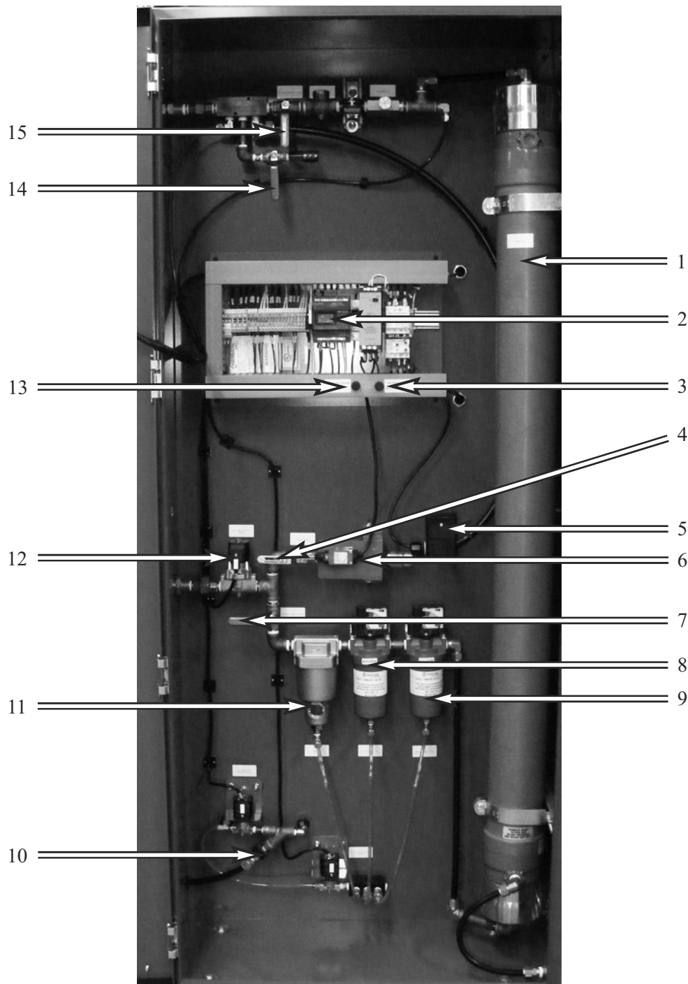
Figure 3: Typical NGP-2200D-M3/M4/M5 Internal View
