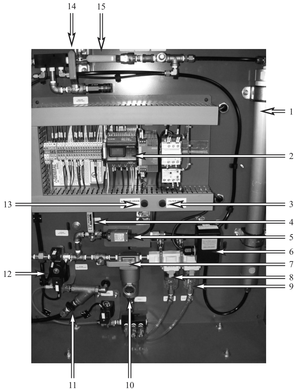
Figure 3: Typical NGP-500D Internal View
